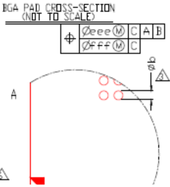
Figure 3- Package Outline Drawing – bottom view
