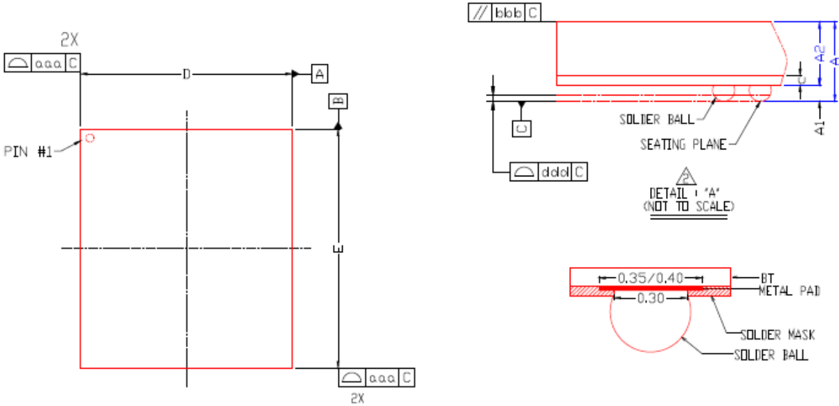
Figure 2 - INAND 7232 Specification Top and Side View (Detail A)
