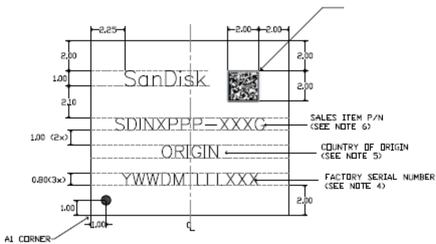
Figure 7 - Product marking 16G-64GB
