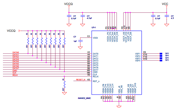
Figure 6 – e.MMC Package Schematics
