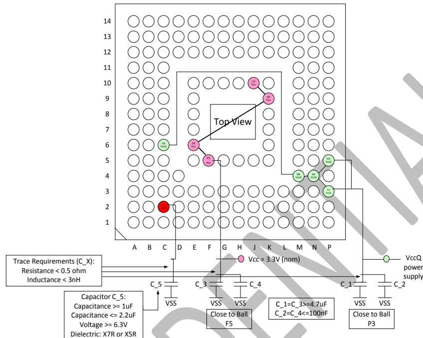
Figure 5 - Recommended Power Domain Connections
